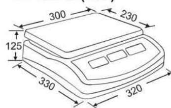
Dimension (mm)
